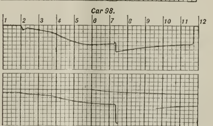
STANDING TEST OF 100-CAR A. S. A. TRAIN. VIRGINIAN RAILWAY, PRINCETON, WEST VIRGINIA, ON JULY 2nd, 1918.
